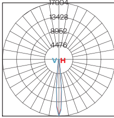
Polar Graph ACCL-27K-10
