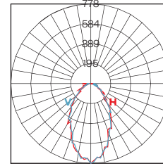
Polar Graph ACCL-27K-60
