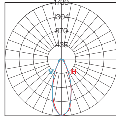
Polar Graph ACCL-27K-30
