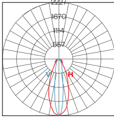
Polar Graph ACCL-27K-60X10
