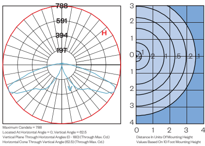
AO25PC-CL-AVI2-700M-SY-27
