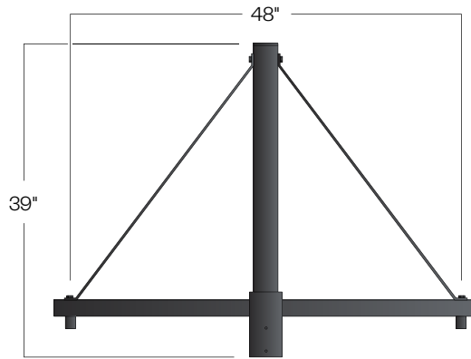
CBR40-2-24-L
