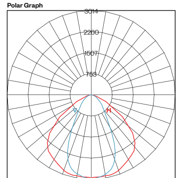
Maximum Candela = 3013.7 Located At Horizontal Angle = -1, Vertical Angle = 1 H - Horizontal Axial Candela V - Vertical Axial Candela
