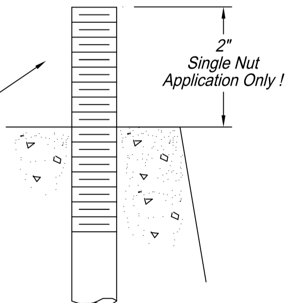
This Is 78920 Template Rotated 45° For 85850-002 Base
