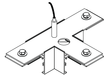
T Connector
