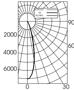
FLOOD 30° DISTRIBUTION LTL # 227549
