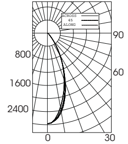
WIDE FLOOD 45° DISTRIBUTION LTL # 227696
