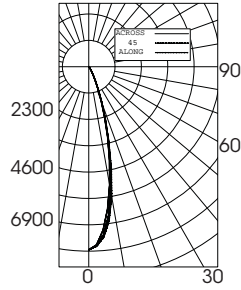
MEDIUM FLOOD 24° DISTRIBUTION LTL # 227550
