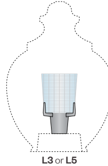
GLASS REFRACTOR Borosilicate glass refractor with IES Type III ( L3 ) or Type V ( L5 ) light distribution can be specified in most fixtures that don't have an integral refractive lens. The refractor can be retrofit in existing fixtures without tools or electrical modifications.
