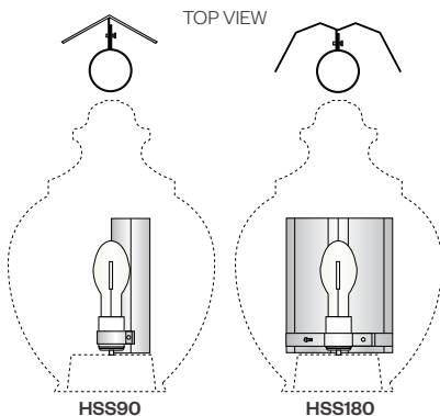
HSS-90 (90 degree cutoff) HSS-180 (180 degree cutoff) House side shields are available to cutoff all direct light through certain horizontal angles. Both models clamp around the socket and are designed to be positioned in the field after installation of the fixture. If ordering for a retrofit application, the socket type must be specified.
