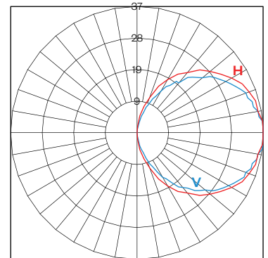
PSCS12/L30 POLAR GRAPH
