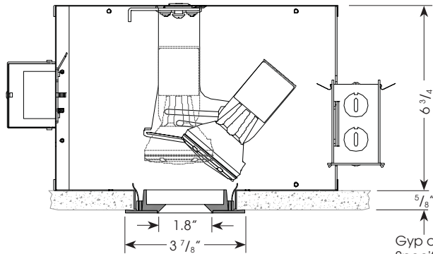
Ceiling Cut Out Dimension: 3 7/8" dia.
