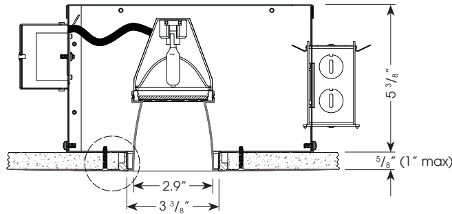
Ceiling Cut Out Dimension: 4 1/16" dia.
