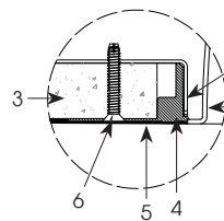
Ceiling Cut Out Dimension: 4 1/16" dia.
