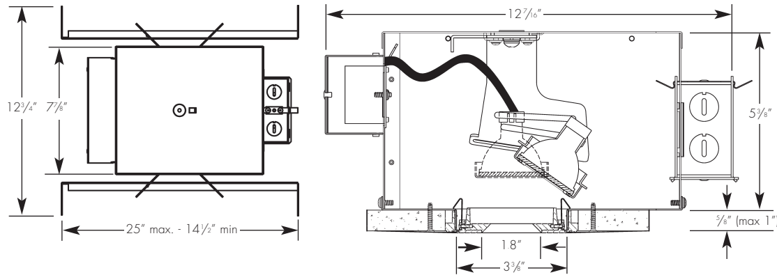
Ceiling cut out dimension: 4 1/16" dia.
