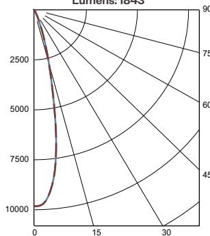
Narrow Flood Distribution, 20° LTL #15682016.01 Lumens: 1843
