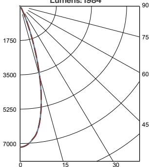
Medium Flood Distribution, 30° LTL #15682016.02 Lumens: 1984
