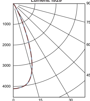
Flood Distribution, 40° LTL #15682016.03 Lumens: 1929
