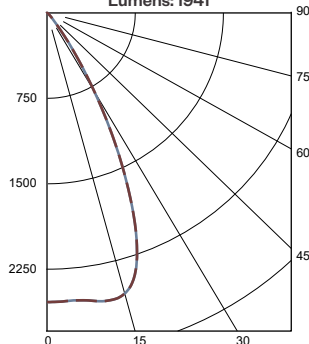
Wide Flood Distribution, 50° LTL #15682016.04 Lumens: 1941
