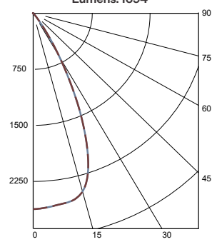
Wide Flood Distribution, 50° LTL #15657122.12 Lumens: 1694
