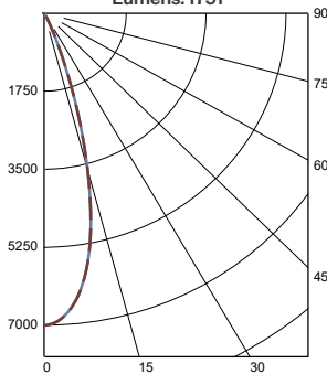
Medium Flood Distribution, 30° LTL #15657122.10 Lumens: 1791
