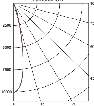
Narrow Flood Distribution, 20° LTL #15657122.09 Lumens: 1617
