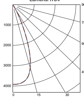
Flood Distribution, 40° LTL #15657122.11 Lumens: 1754
