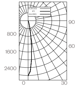
WIDE FLOOD (WF) 45° DISTRIBUTION LTL # 227696
