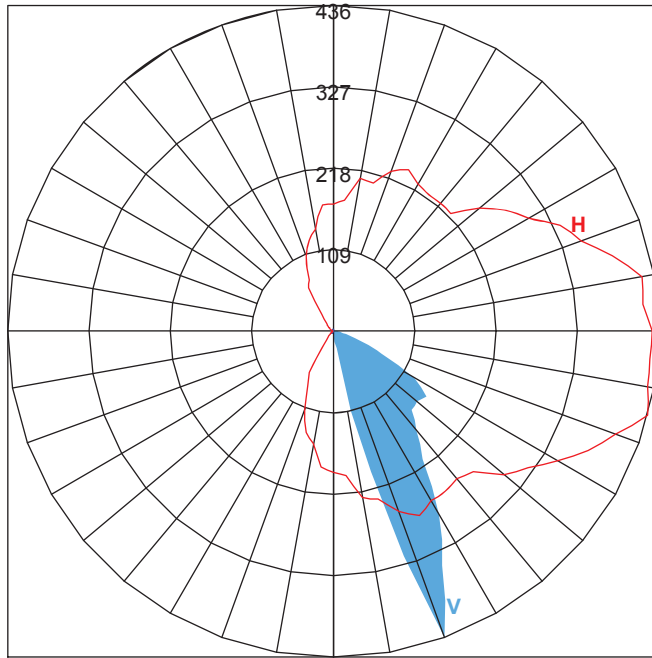
AB5-34-180 POLAR GRAPH
