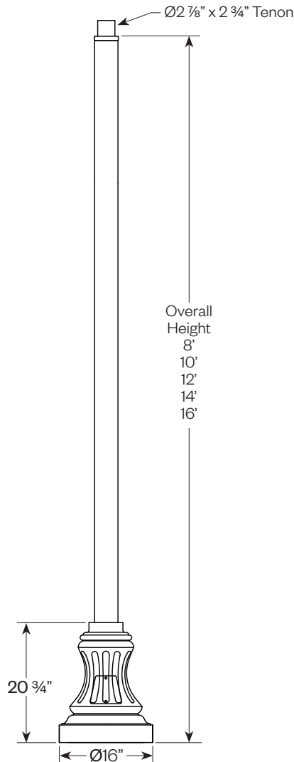
Smooth Shaft
