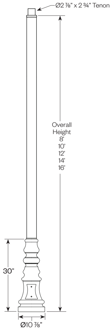
Smooth Shaft
