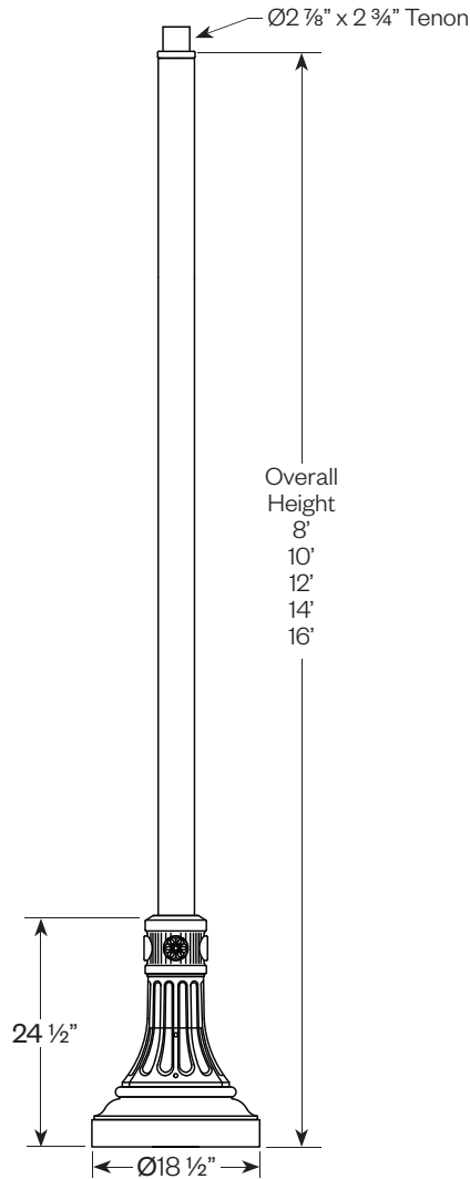
Smooth Shaft
