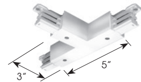
TEK39 T Connector (feedable) (adjustable right polarity) TEK40 T Connector (feedable) (adjustable left polarity)
