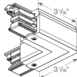
XTS34 - L Connector, feedable, adjustable universal polarity
