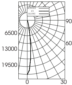
Narrow Flood 16° Distribution LTL # 227548 Lumens: 2,221
