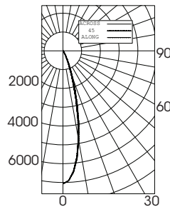
Flood 30° Distribution LTL # 227549 Lumens: 1,821
