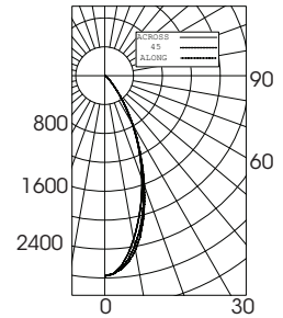
Wide Flood 45° Distribution LTL # 227696 Lumens: 1,825
