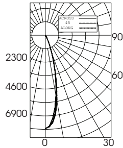
Medium Flood 24° Distribution LTL # 227550 Lumens: 2,052
