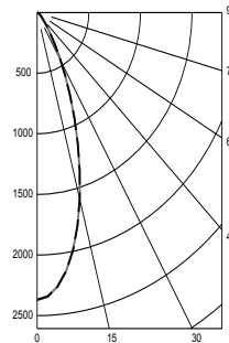
Wide Flood (WF) Distribution LTL # 860529 Lumens: 1,278
