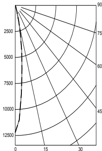
Spot (SP) Distribution LTL #855377 Lumens: 1,369
