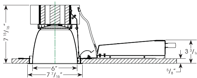
Ceiling Cut Out Dimension: 7" dia.
